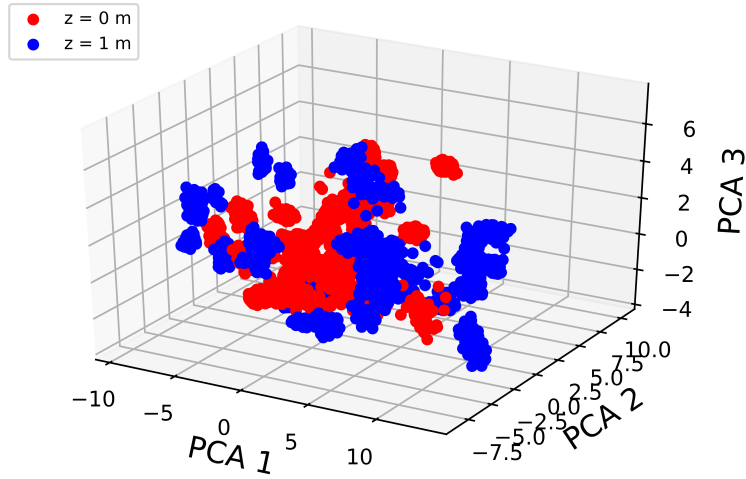
Fig. 4. Illustration of PRF spectrum with reduced dimensionality by PCA. The red and blue dots indicate that spectrum data was collected at 0 and 1 m from the ground, respectively.
