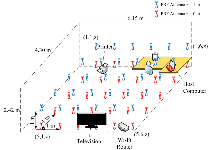
Fig. 3. Illustration of an indoor living room scenario is used to collect PRF data at 60 positions. The red and blue antennas are represented as 0 and 1 meters from the bottom of the antenna to the ground, respectively. Other potentially disturbing objects and human are also marked.
